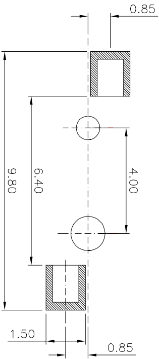
PCB LAND DIMENSION
