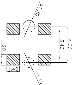
PCB LAND DIMENSION
