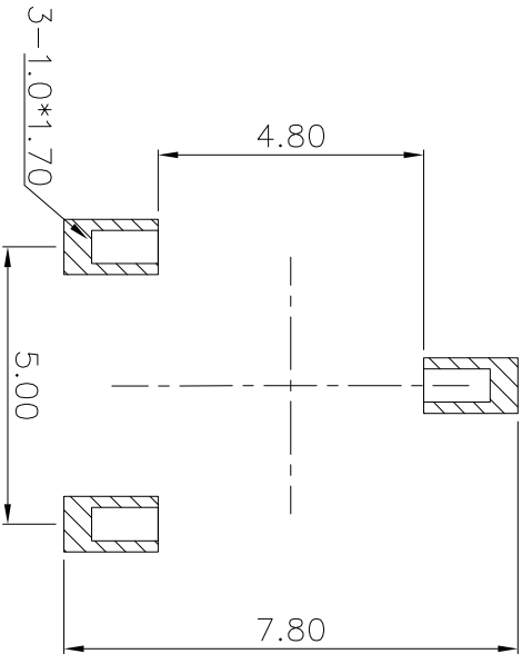
LAYOUT
