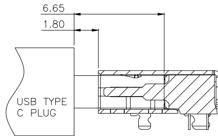
AFTER MATING
