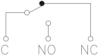
Circuit Diagram
