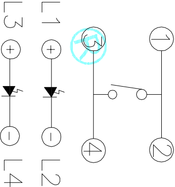
Circuit Diagram
