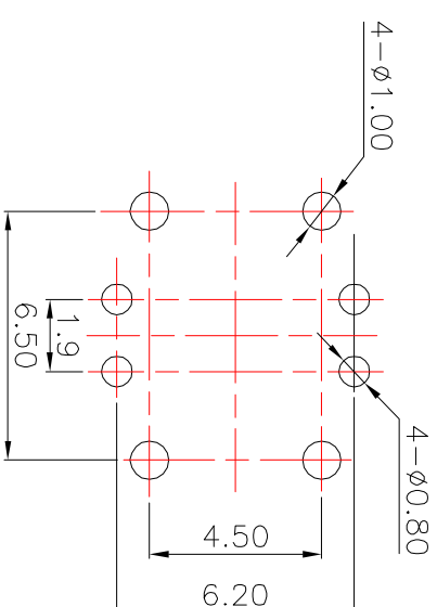
PCBLayout(Pattern Side)
