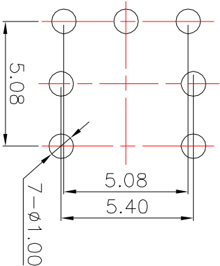
PCBLayout(Pattern Side)
