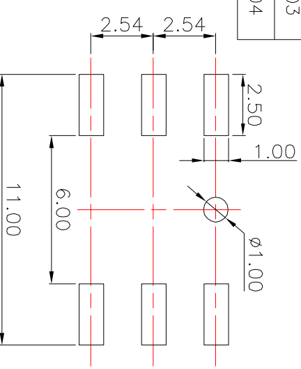
PCBLayout(Pattern Side)
