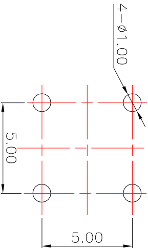
PCBLayout(Pattern Side)
