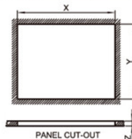
PANEL CUT-OUT
