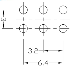
P.C.B LAYOUT BOTTOM VIEW CIRCUIT DIAGRAM
