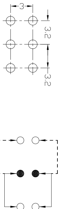
P.C.B LAYOUT BOTTOM VIEW
